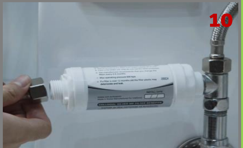
Connect Braided Hose to Filter
